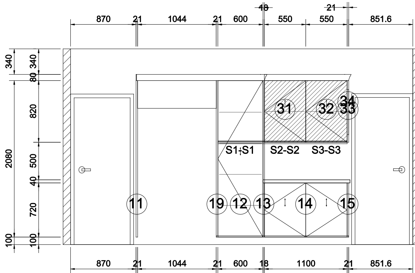
A View elevation drawing
