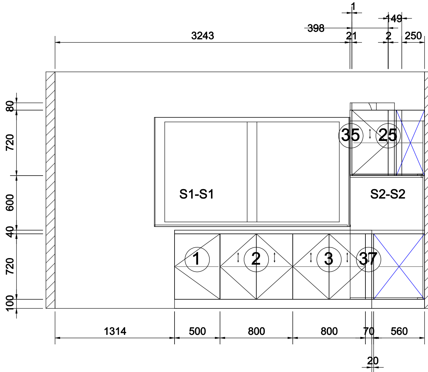
B View elevation drawing
