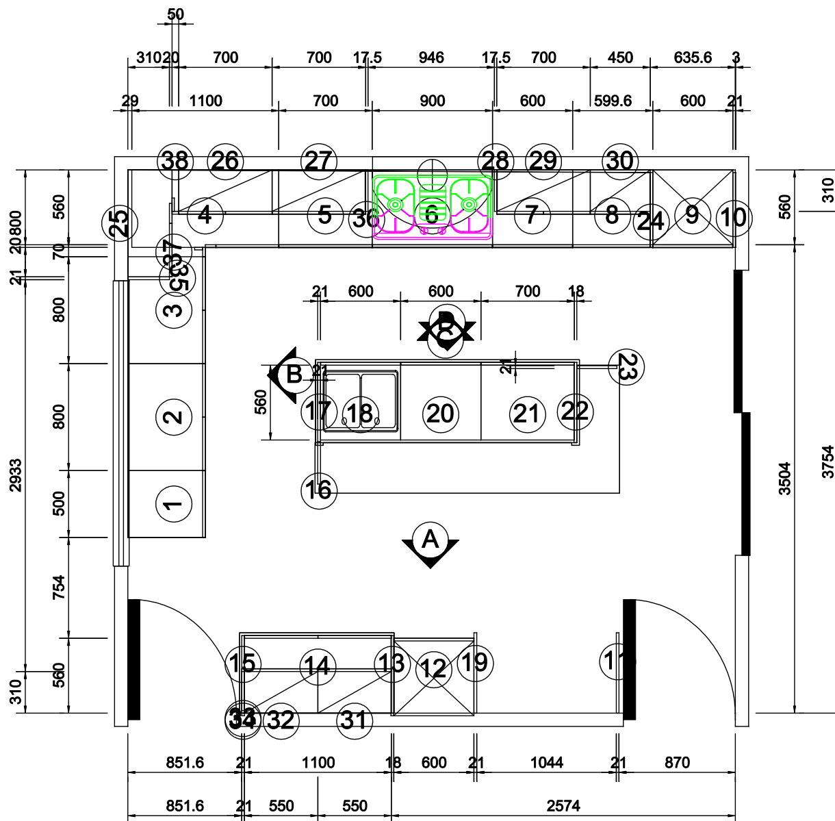
Plan drawing
