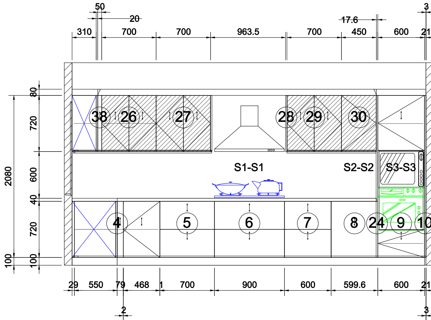
C View elevation drawing
